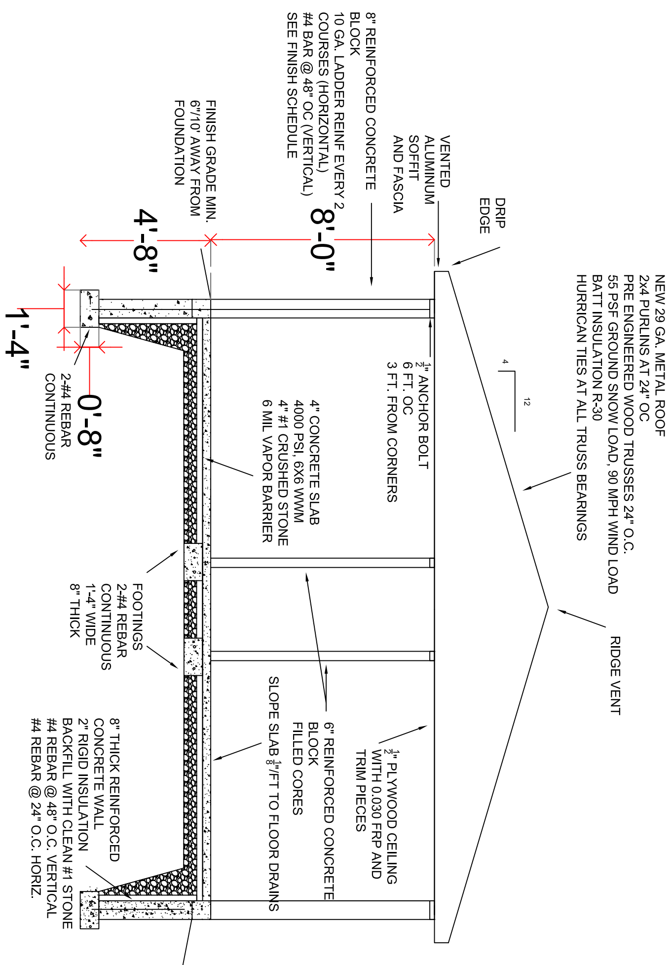
SHOWERHOUSE SECTION
